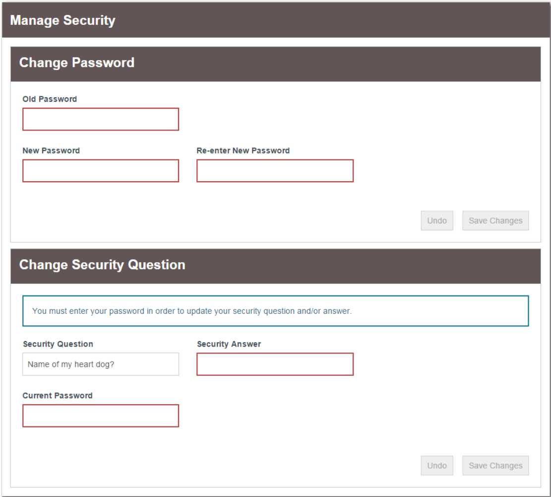
Figure 5.4 – Manage Security Page
